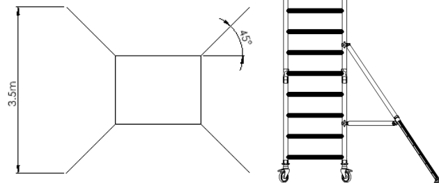
STABILISERS—S3
