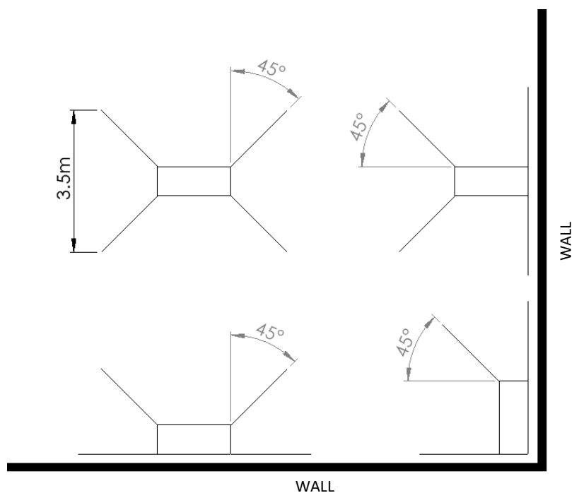
Static Stabiliser maximum platform height of 4.2m
